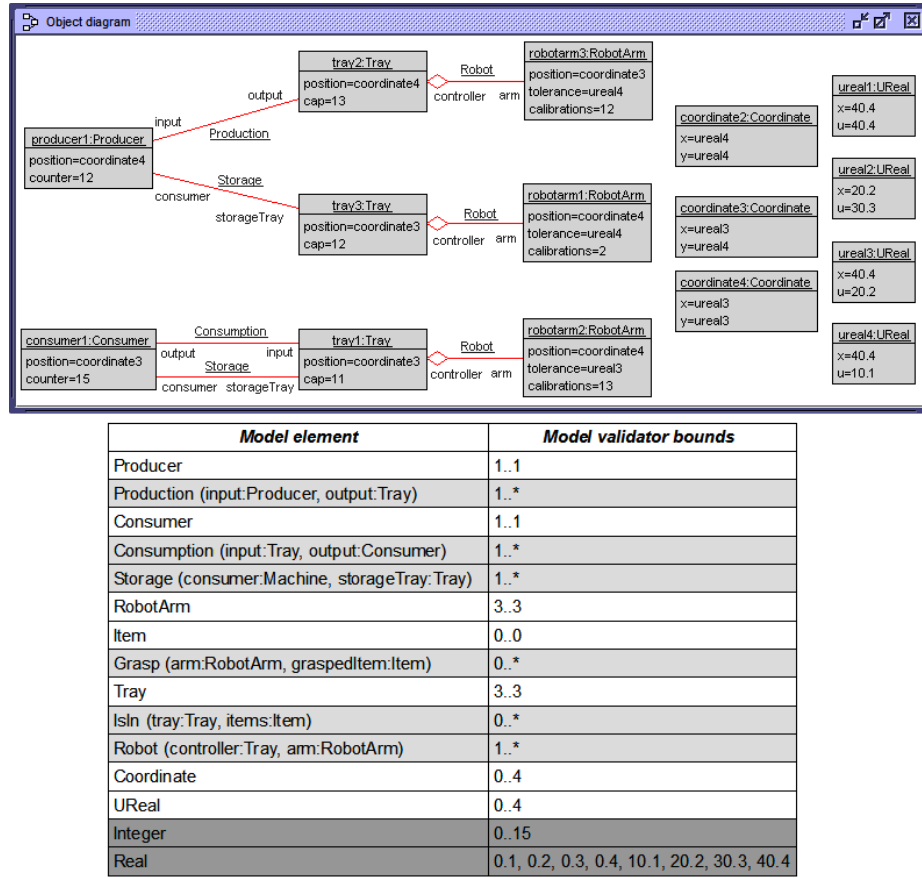
Fig. 8. Generated test case for Producer-Consumer-Tray configuration.
